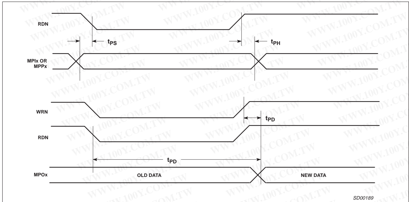
Figure 7. Port Timing
