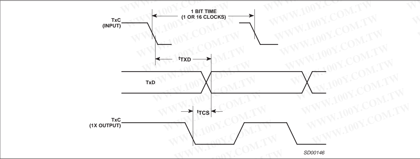
Figure 10. Transmit Timing
