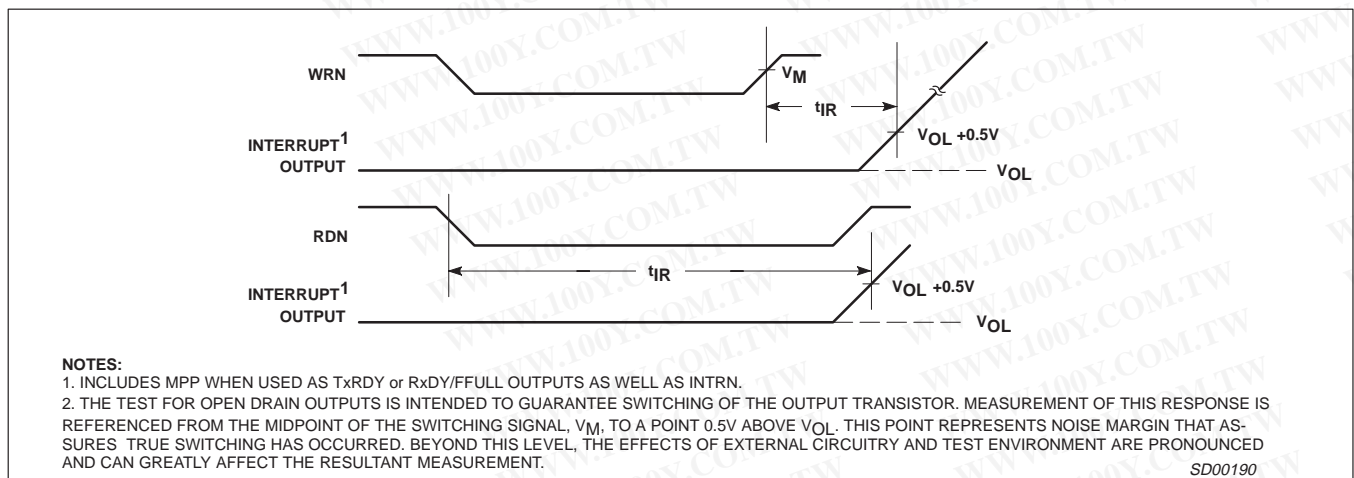
Figure 8. Interrupt Timing
