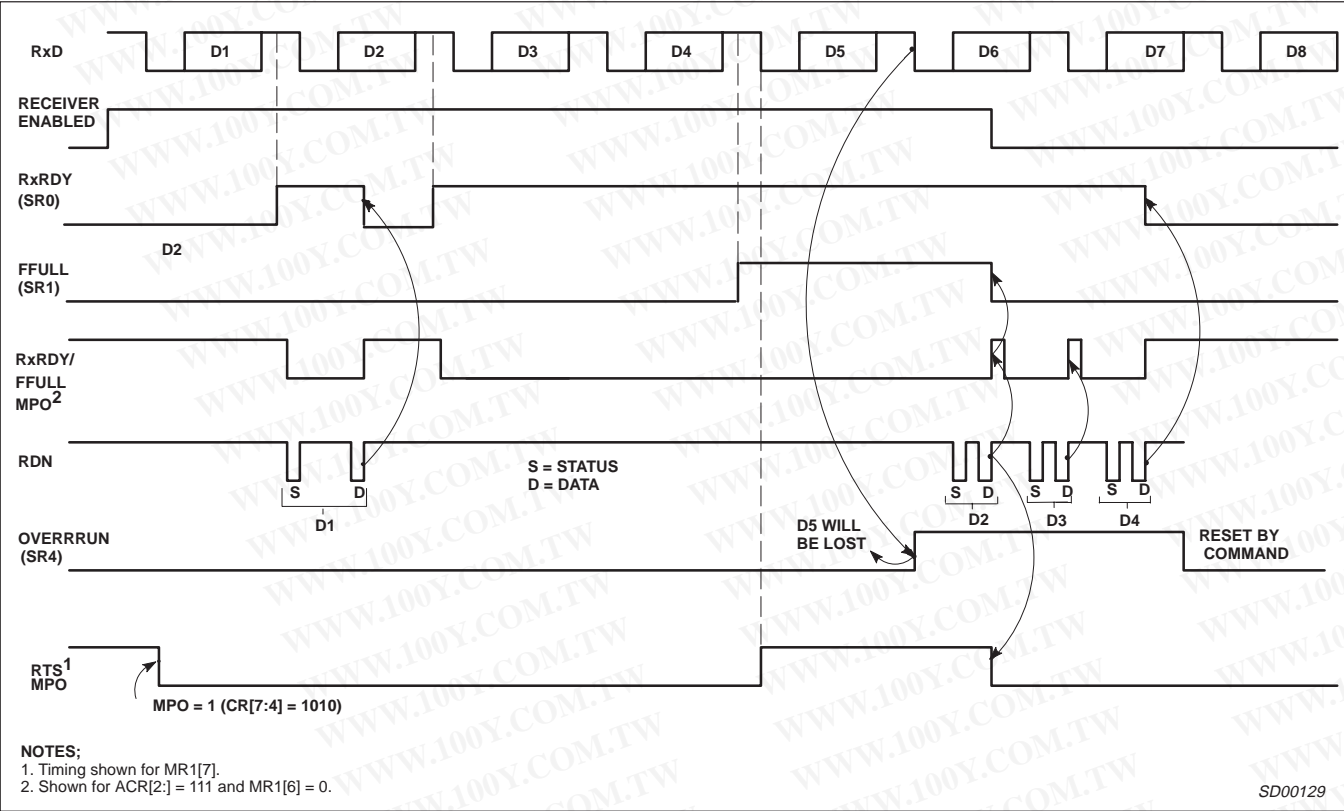
Figure 13. Receiver Timing
