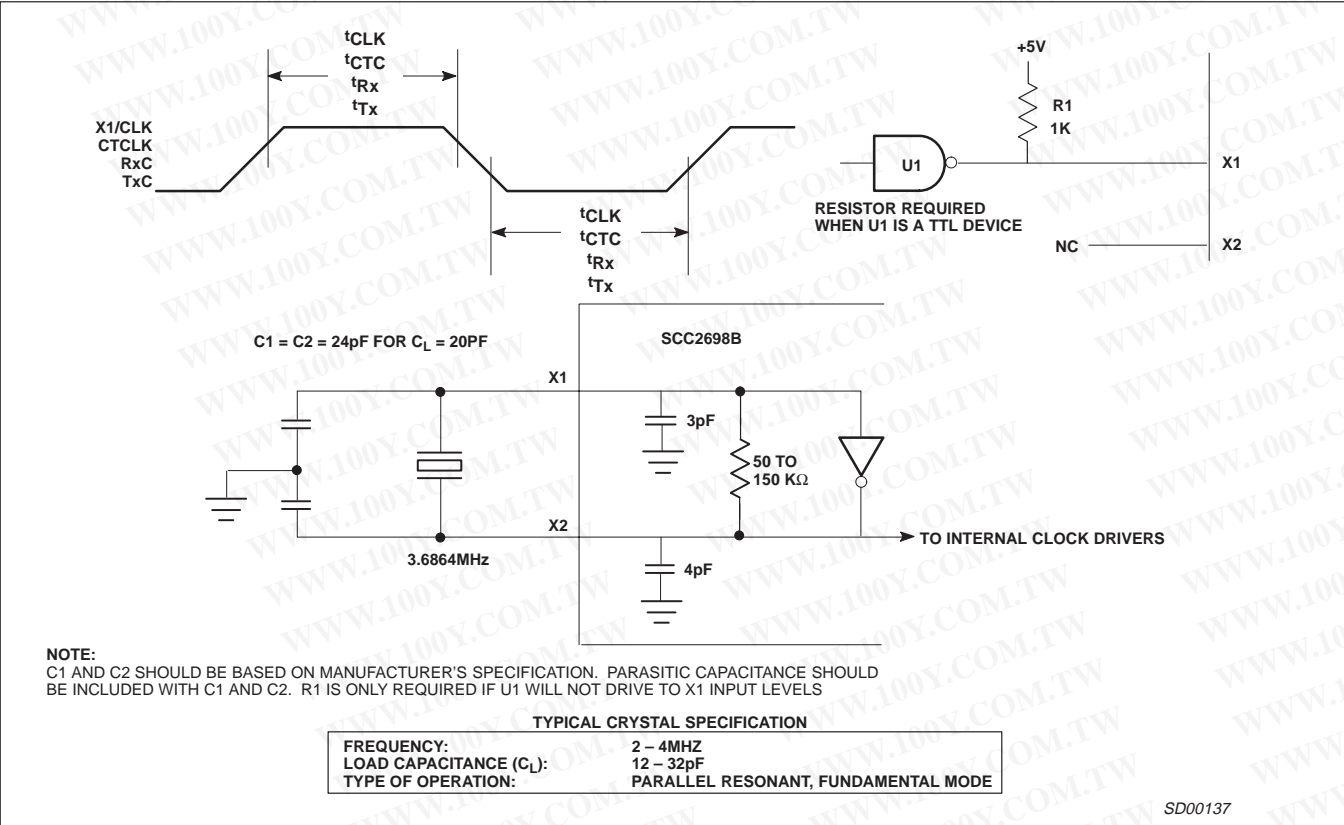
Figure 9. Clock Timing
