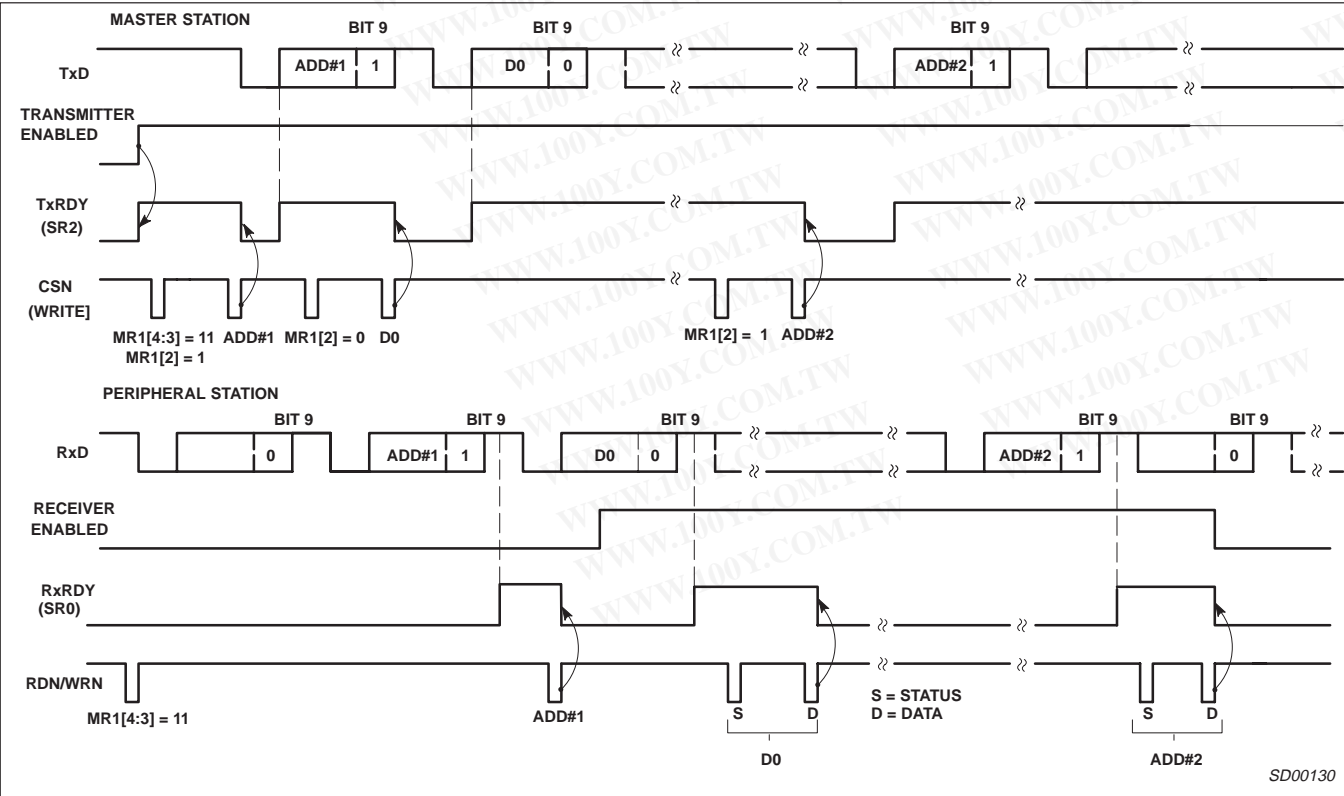
Figure 14. Wake-Up Mode
