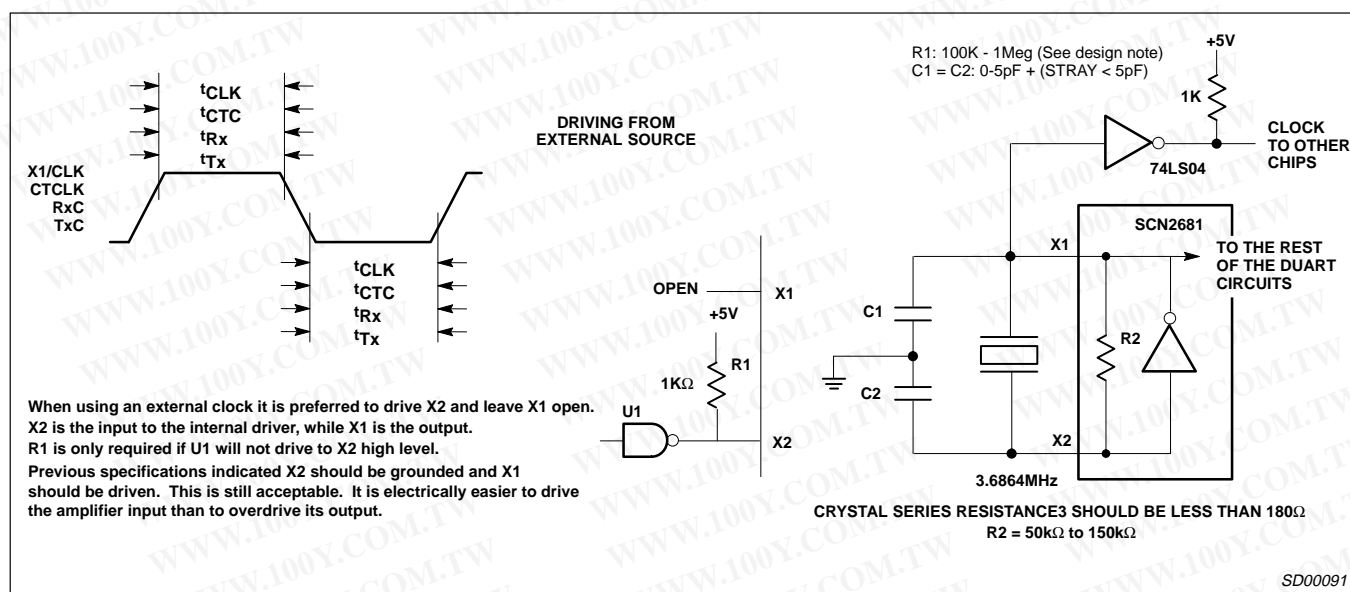
Figure 5. Clock Timing
