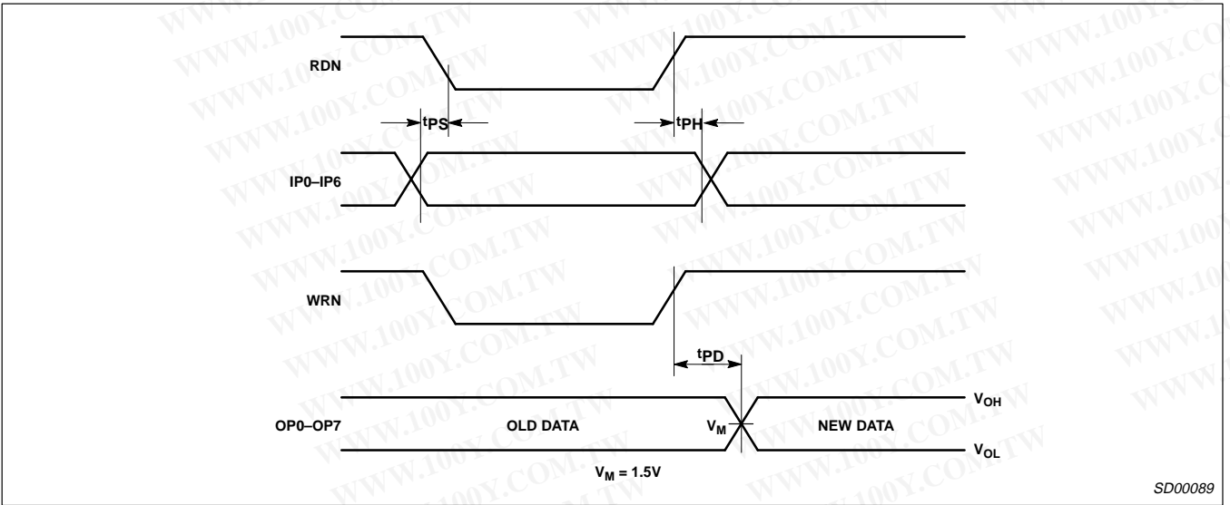
Figure 3. Port Timing
