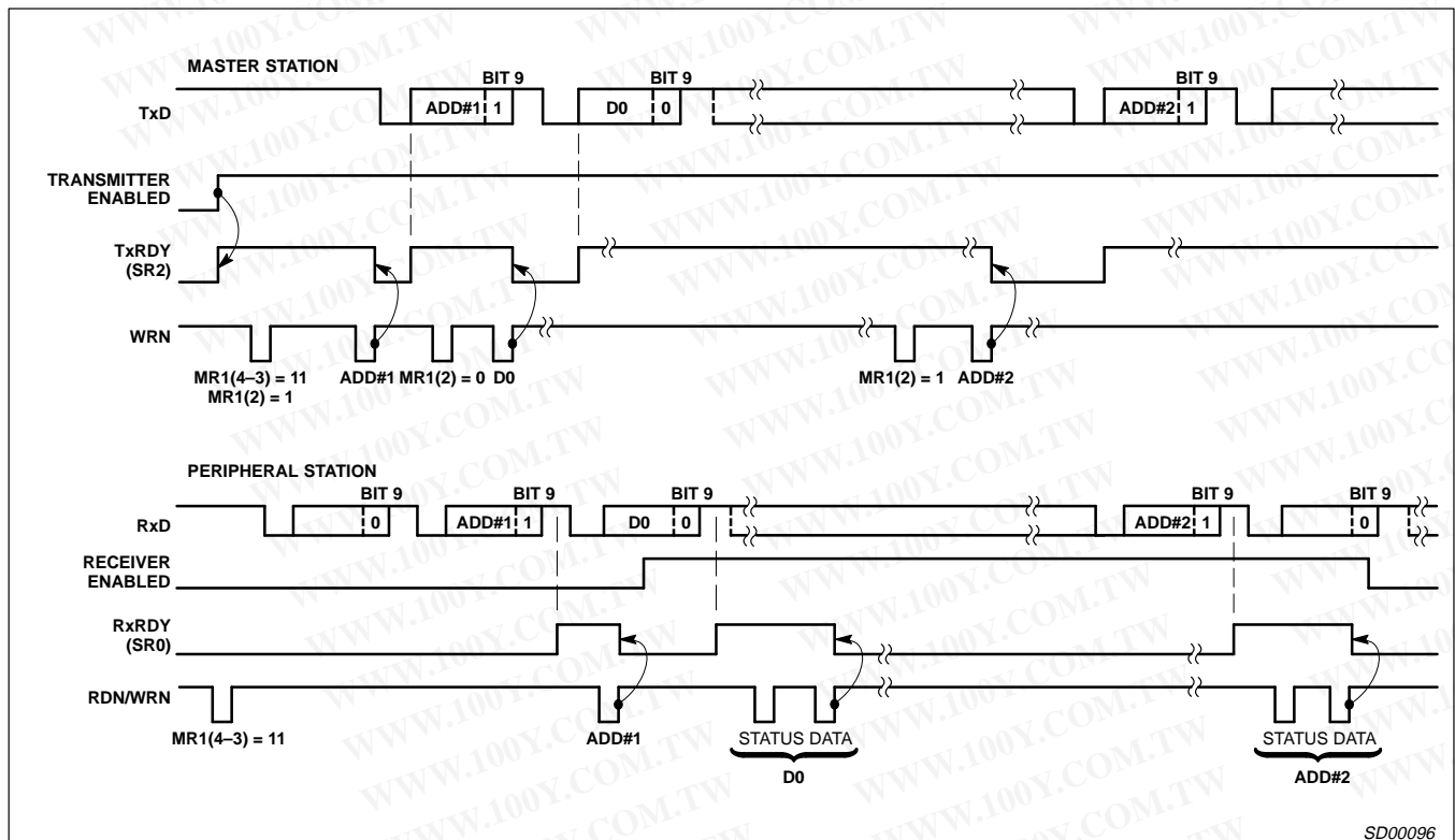
Figure 10. Wake-Up Mode
