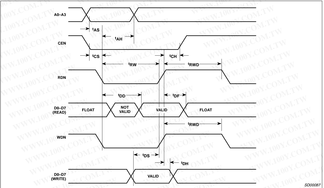
Figure 2. Bus Timing
