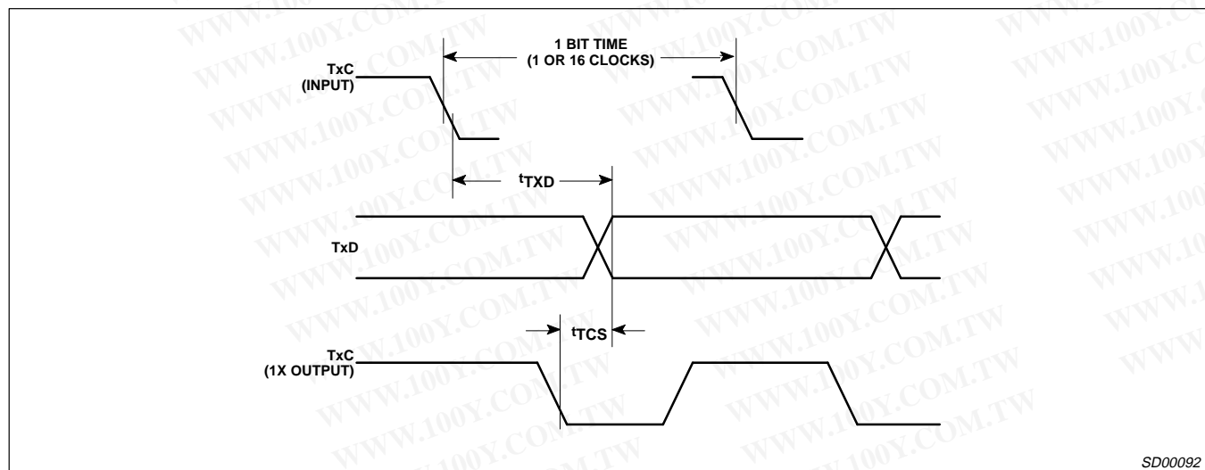
Figure 6. Transmit
