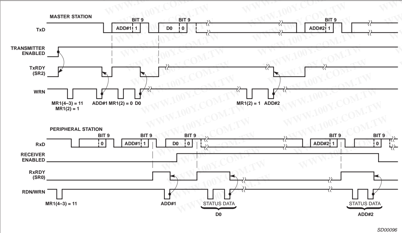
Figure 12. Wake-Up Mode
