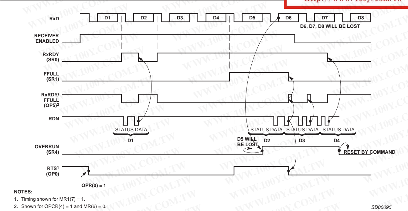
Figure 11. Receiver Timing
