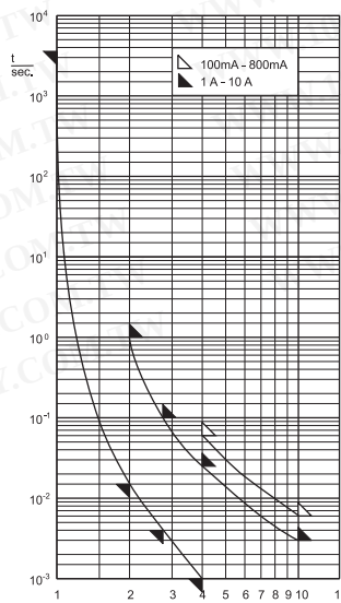
Part No. 70 001 40
