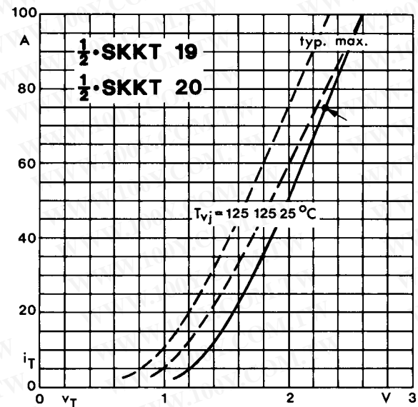
Fig. 8 On-state characteristics
