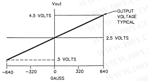
TRANSFER CHARACTERISTICS V S 5.0 VDC
