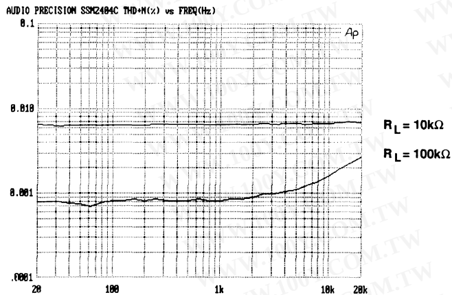
Figure 1. THD+N vs. Frequency ( V_S = \pm 12V , V_A = 2V rms, with 80 kHz Filter)
