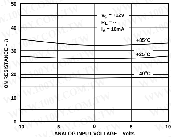
Figure 12. ON Resistance vs. Analog Voltage
