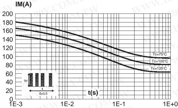
Fig. 3-1: Non repetitive surge peak forward current versus overload duration (maximum values, per diode) (TO-220AB, D 2 PAK, SOT-93 and TO-247).
