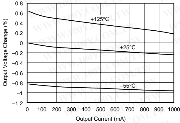
OUTPUT VOLTAGE CHANGE vs I_{\text{OUT}} (V_{\text{IN}} = V_{\text{OUT}} + 1\text{V}, \text{Output Voltage \% Change} Referred to I_{\text{OUT}} = 10\text{mA} at +25^\circ\text{C} )
