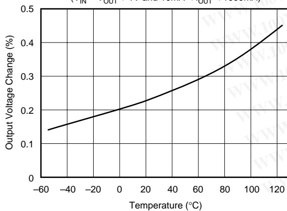
LOAD REGULATION vs TEMPERATURE ( V_{\text{IN}} = V_{\text{OUT}} + 1\text{V} and 10\text{mA} < I_{\text{OUT}} < 1000\text{mA} )
