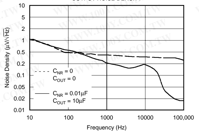
OUTPUT NOISE DENSITY
