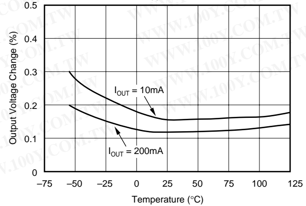
LINE REGULATION vs TEMPERATURE (V_{\text{IN}} = V_{\text{OUT}} + 1\text{V to } 16\text{V})
