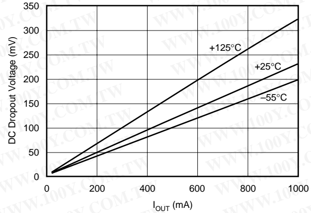
DC DROPOUT VOLTAGE vs I_{\text{OUT}}
