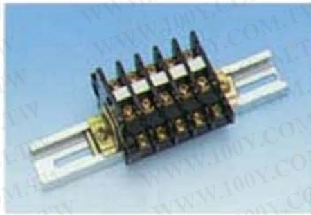
TBC-N RAIL-MOUNT TYPE
