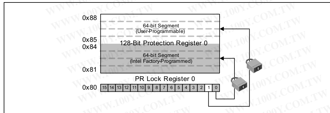
Figure 14. Protection Register Mapping
