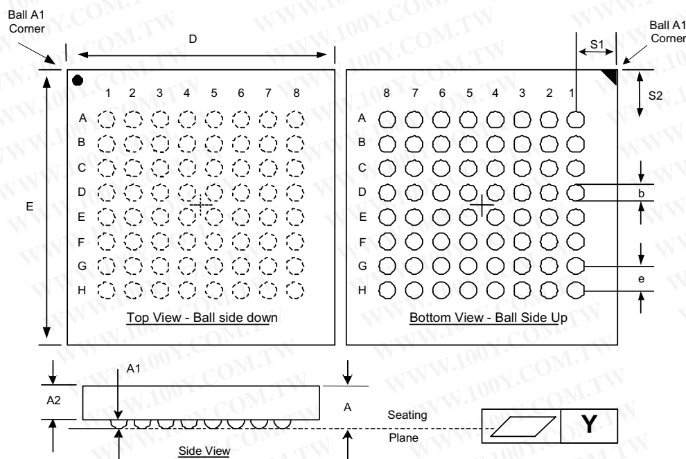
Figure 3. Easy BGA Package Drawing and Dimension
