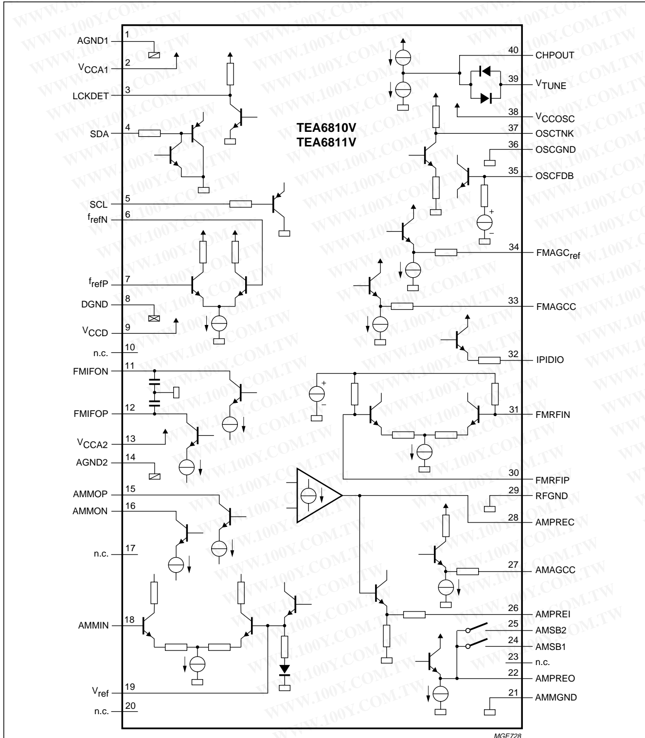
Fig.7 Internal pin configuration.
