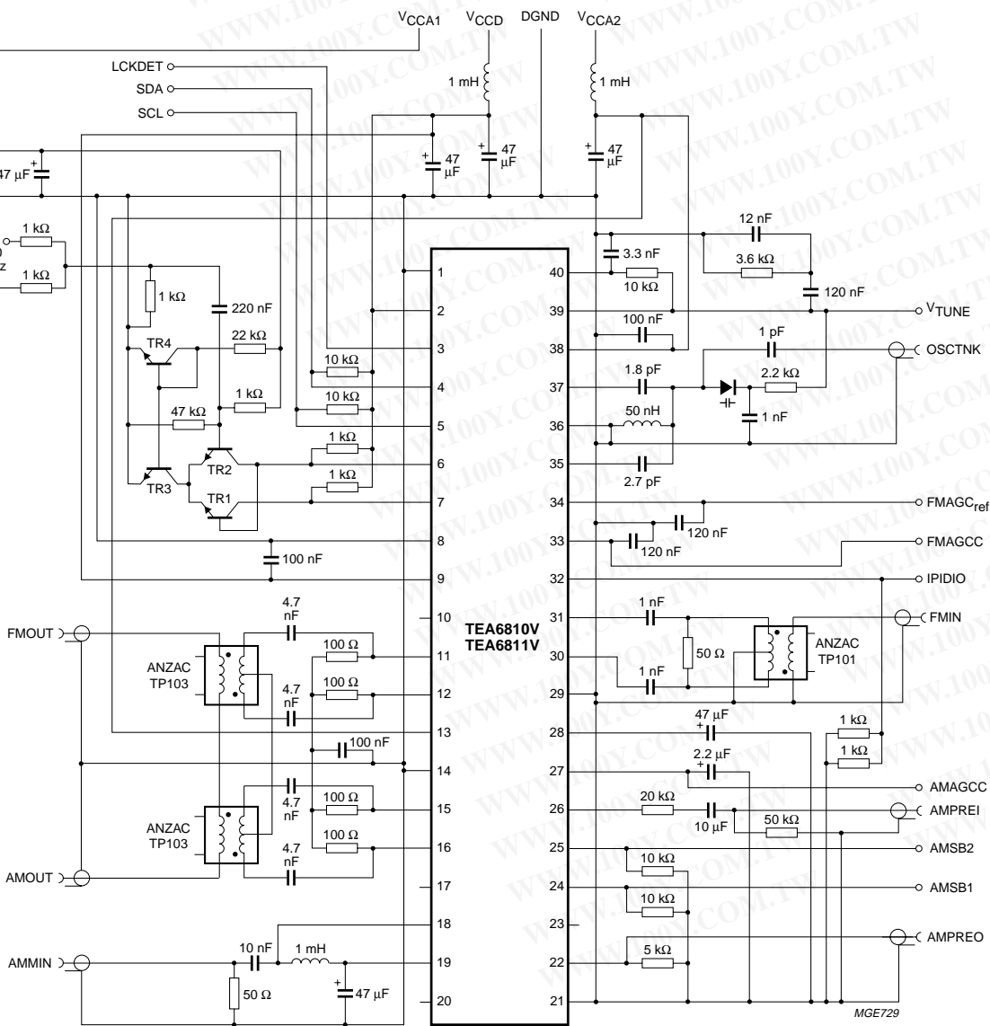
Fig.8 Test board diagram.
