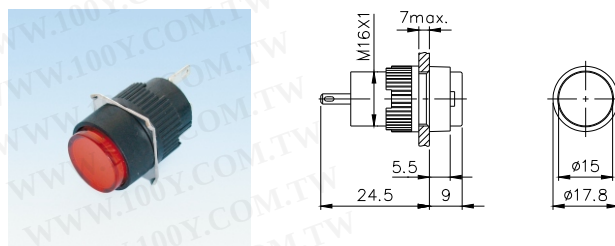
TN16-PIS/PLS/PNS
