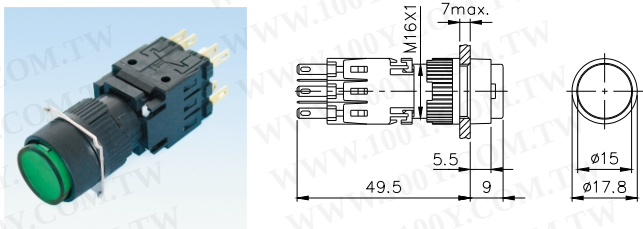
TN16-AIS/ALS/ANS TN16-MIS/MLS/MNS
