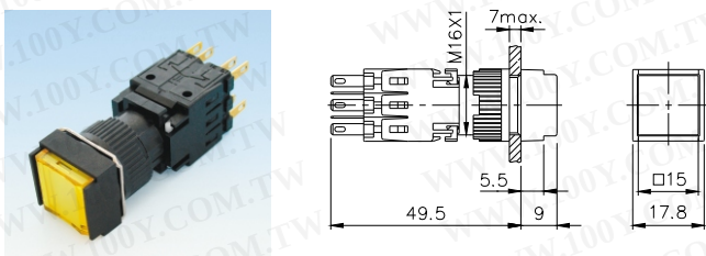
TN16-AIL/ALL/ANL TN16-MIL/MLL/MNL
