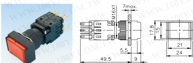
TN16-AIL/ALL/ANL TN16-MIL/MLL/MNL
