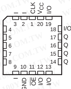
TIBPAL16R4' C SUFFIX ... FN PACKAGE M SUFFIX ... FK PACKAGE (TOP VIEW)
