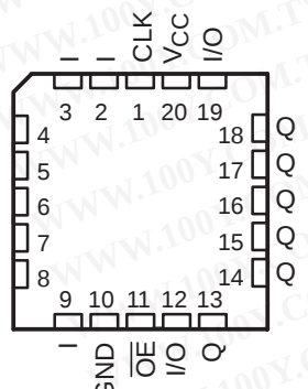
TIBPAL16R6' C SUFFIX ... FN PACKAGE M SUFFIX ... FK PACKAGE (TOP VIEW)
