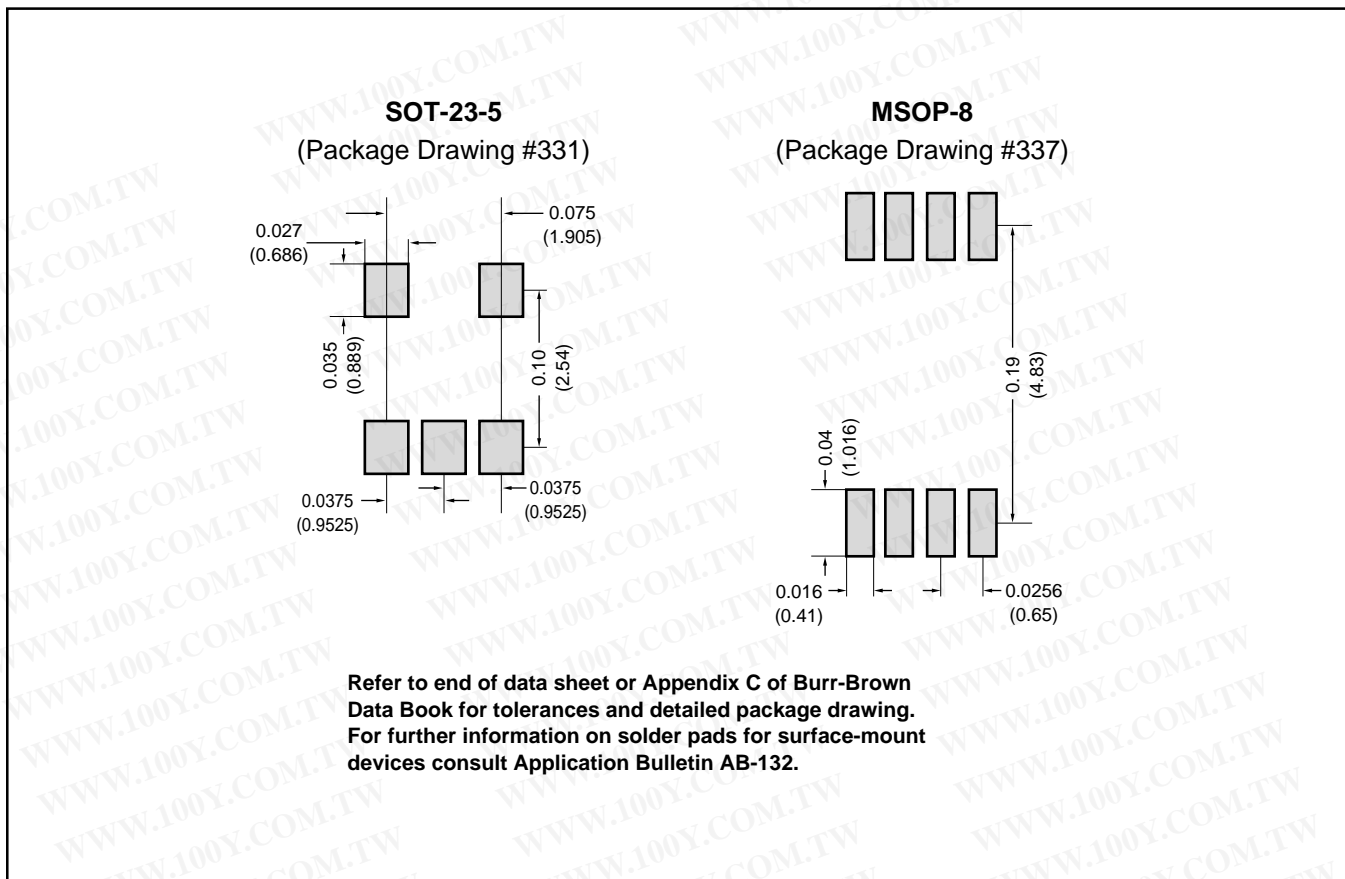
FIGURE 4. Recommended SOT-23-5 and MSOP-8 Solder Footprints.
