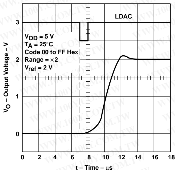
POSITIVE RISE AND SETTLING TIME
