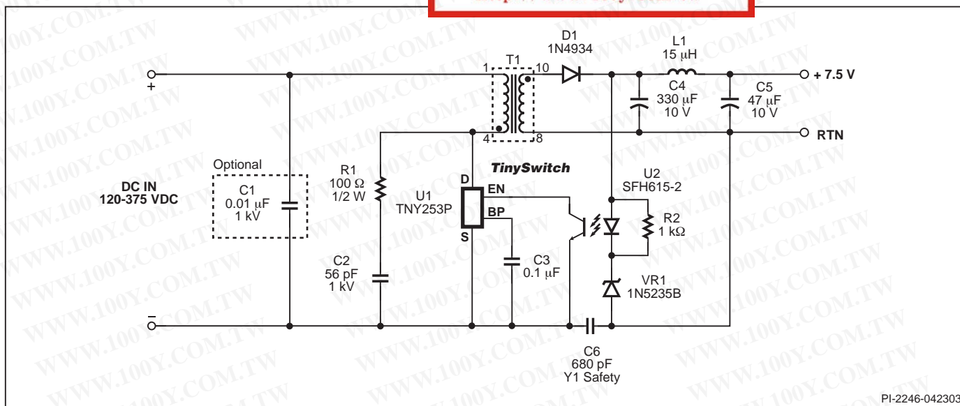
Figure 9. 1.3 W TV Standby Circuit using TNY253.
