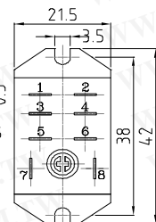
Bracketed Cover Type
