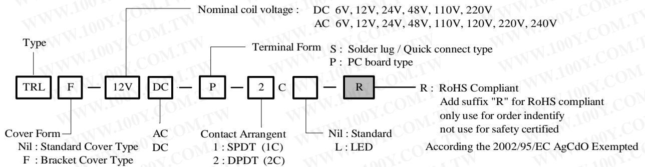
Bracketed Cover Type
