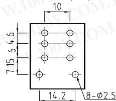
DPDT (2C)
