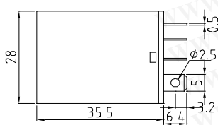
Standard Cover Type
