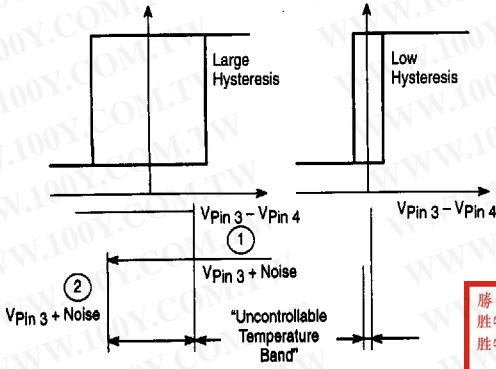
Figure 5. Effects of Inputs Comparator Hysteresis
