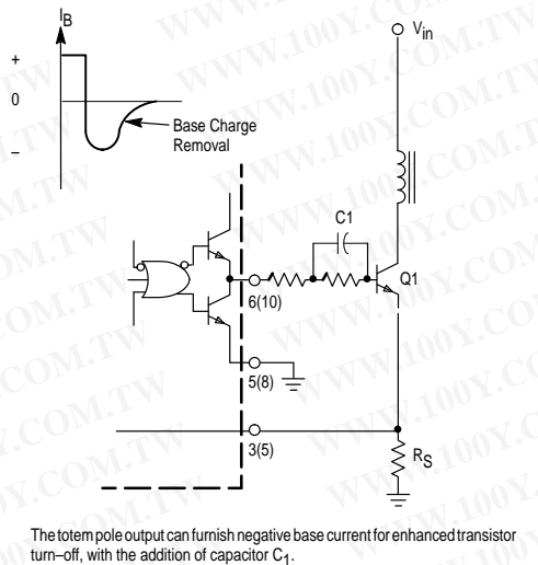
Figure 28. Bipolar Transistor Drive
