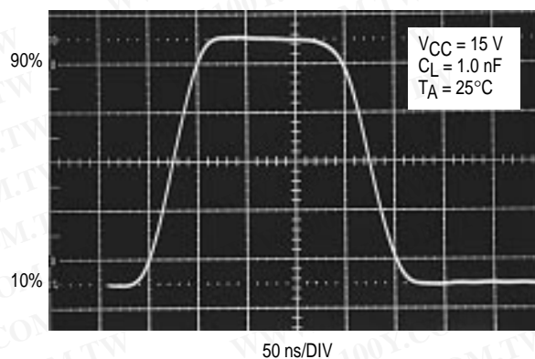
Figure 14. Output Waveform
