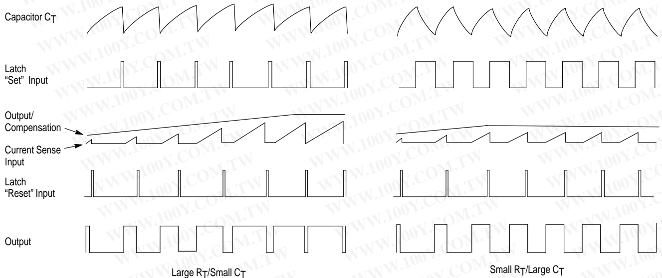
Figure 18. Timing Diagram
