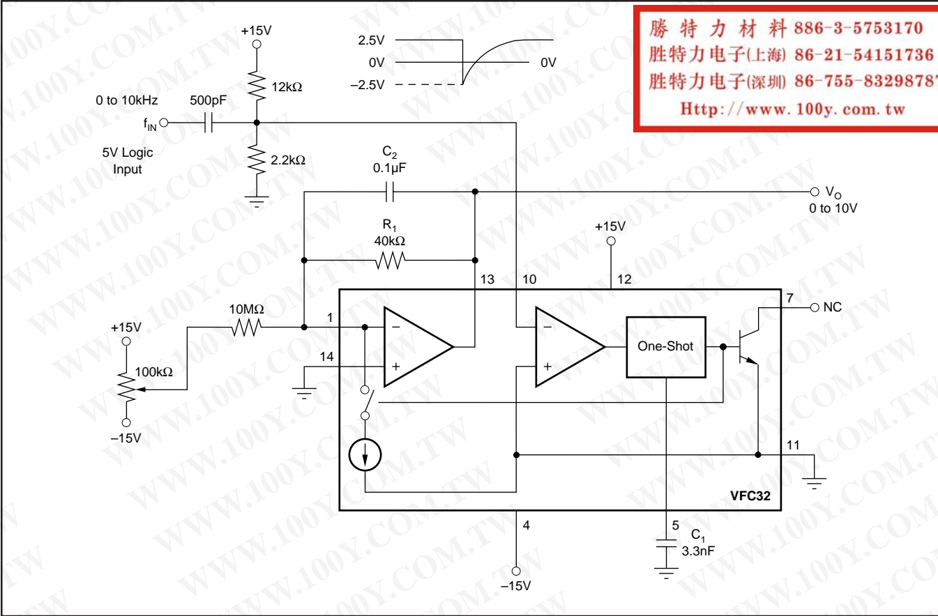
FIGURE 4. Frequency-to-Voltage Converter Circuit.
