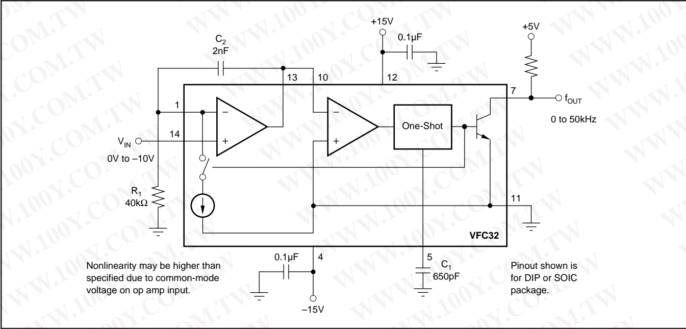
FIGURE 5. V/F Converter—Negative Input Voltage.
