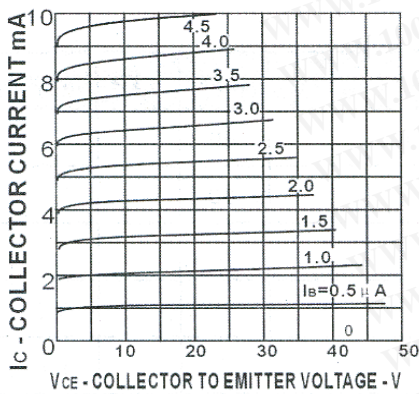
FIG.3 Collector Current vs Collector to Emitter Voltage
