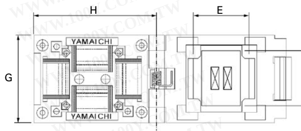
Outline Clamshell Socket Dimensions
