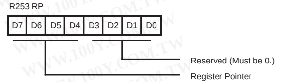
Figure 35. Register Pointer FD H : Read/Write)
