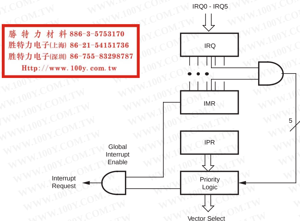
Figure 16. Interrupt Block Diagram
