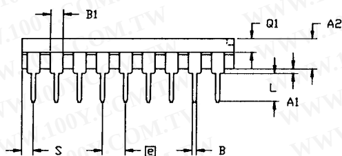
Figure 37. 18-Pin DIP Package Diagram
