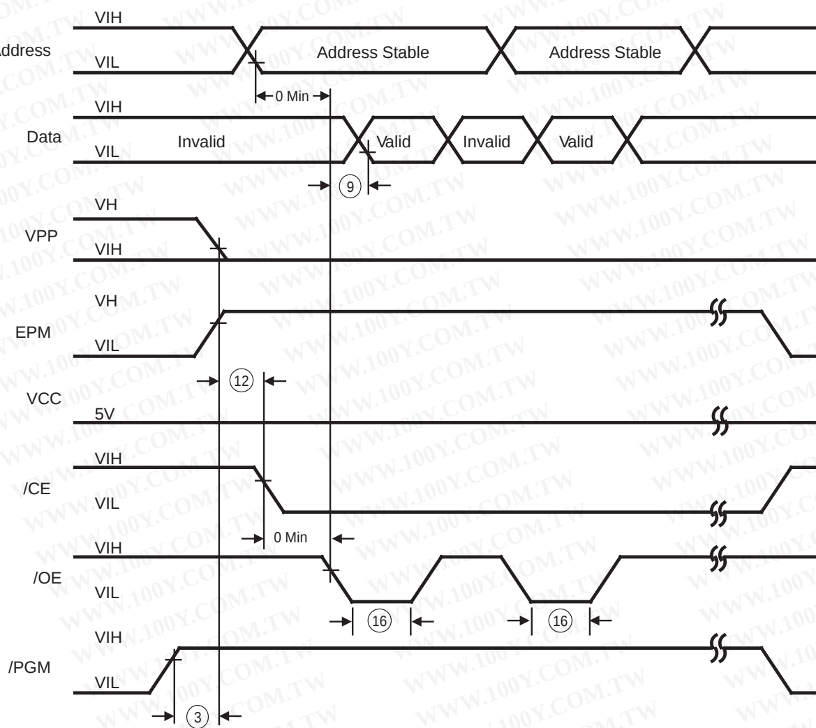
Figure 20. Z86E02 Programming Waveform (EPROM Read)
