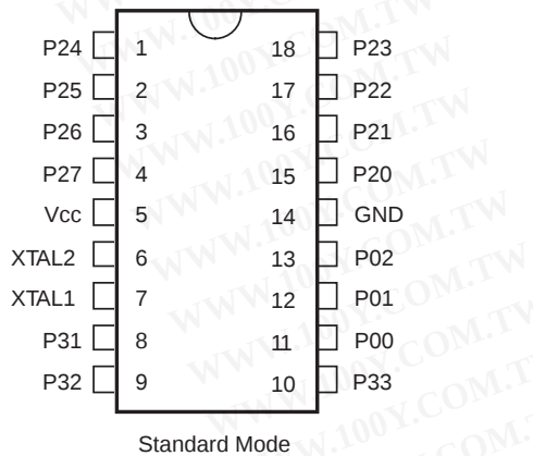
Figure 3. 18-Pin Standard Mode Configuration
