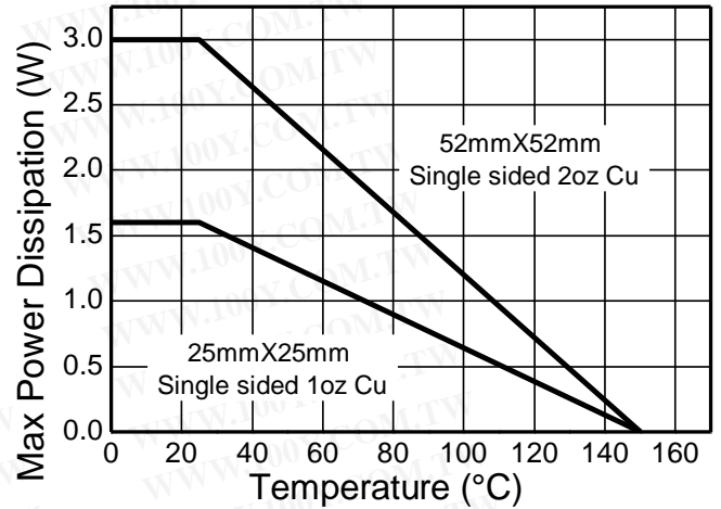
Derating Curve
