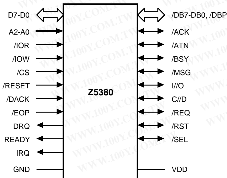
Figure 2. Logic Symbol
