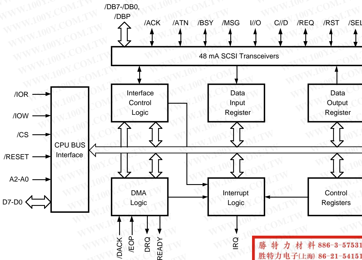
Figure 1. Z5380 Block Diagram
