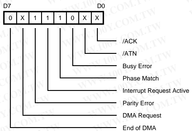
Figure 20. Bus and Status Register
