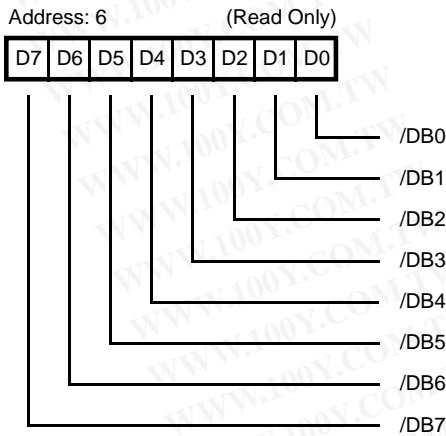
Figure 32. Input Data Register
