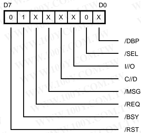
Figure 23. Current SCSI Bus Status Register
