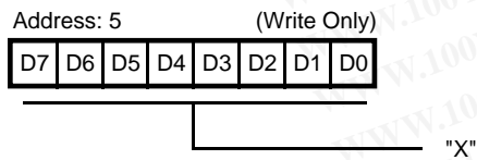
Figure 39. Start DMA Send
