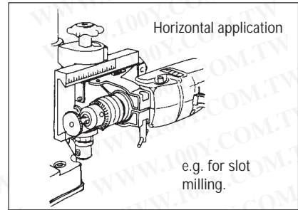
Head may be tilted through 90°.
