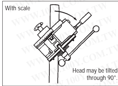
Head feed adjustable to fine feed by means of lever.
