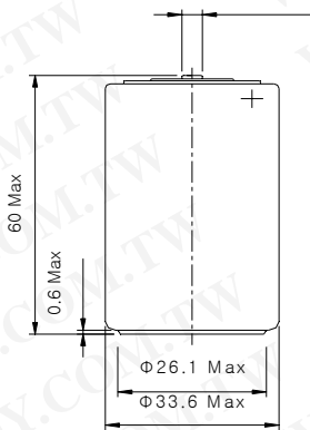
Dimemions in mm Φ4.0 Max
