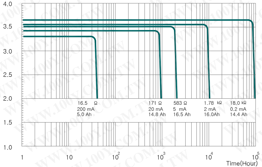
Voltage(V) DISCHARGE CHARACTERISTICS AT +20°C
