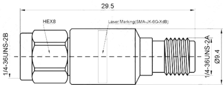
SMA Male To Female 2W 6G 2dB Fixed Attenuator
