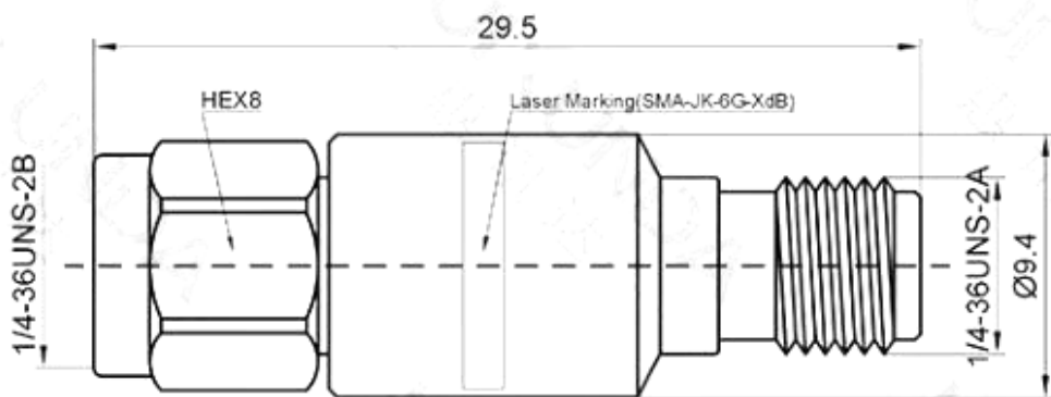
SMA Male To Female 2W 6G 6dB Fixed Attenuator
