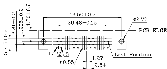
PCB Layout (A)
