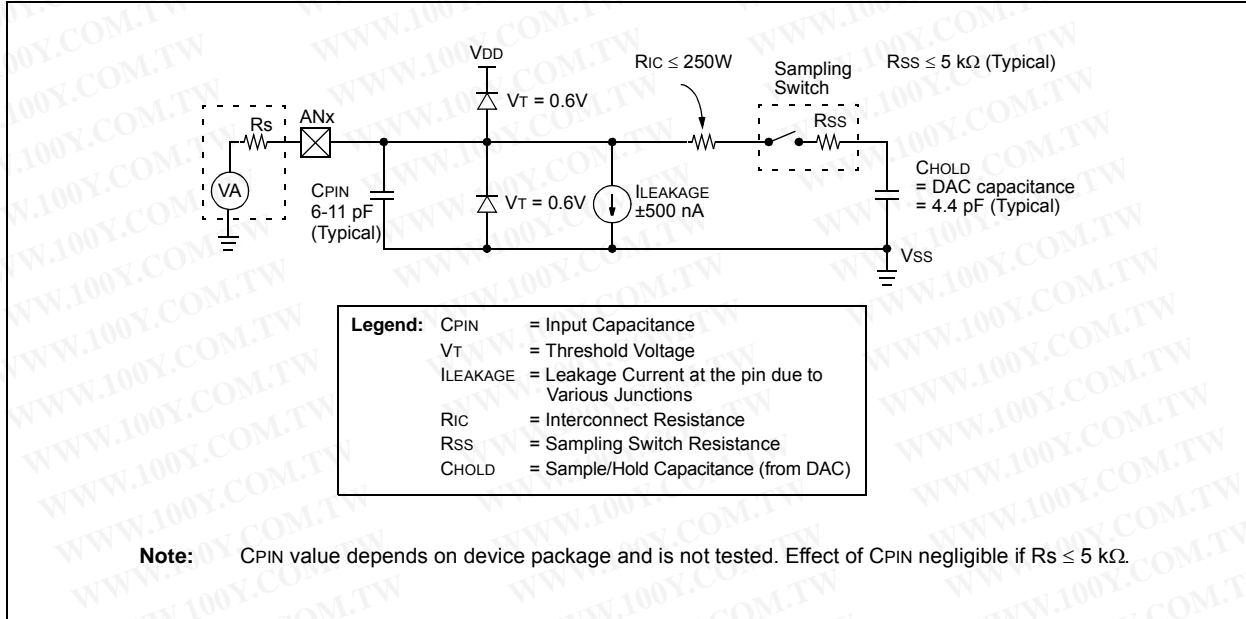
FIGURE 19-2: 10-BIT A/D CONVERTER ANALOG INPUT MODEL
