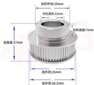
40齿内孔12mm(带宽6mm)
