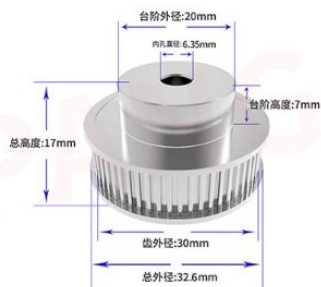
48齿内孔6.35mm(带宽6mm)
