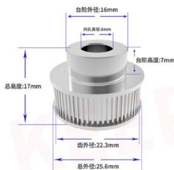
36齿内孔8mm(带宽6mm)
