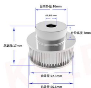
36齿内孔5mm(带宽6mm)
