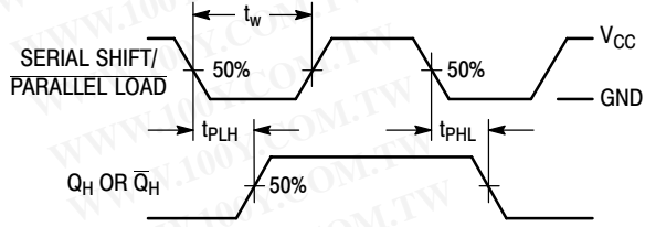
Figure 4. Parallel-Load Mode
